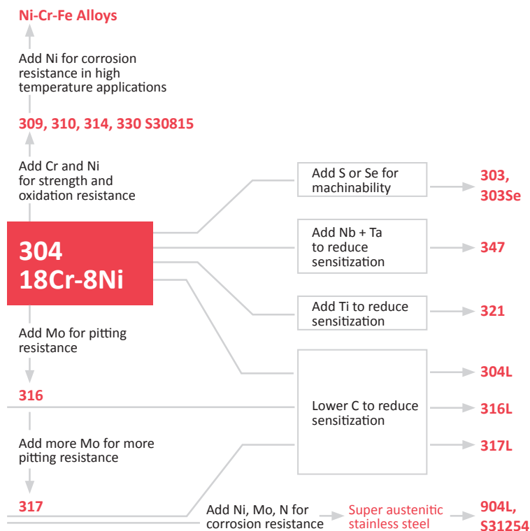
Figure 4. The relationship between the various 300 series austenitic grades (Courtesy Kappa Associates International [2]).
